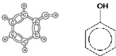
Fenol
