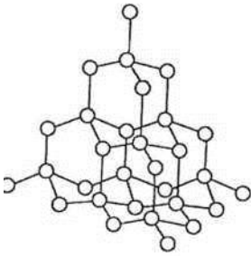
Diamant
