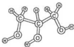
Glycerol
